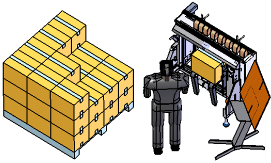
Basic PackPod layout product infeed on top
