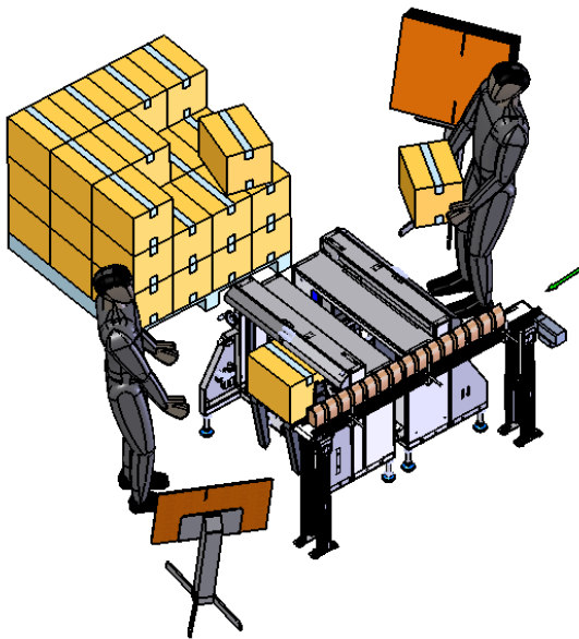
2 operator layout w/ conveyor
